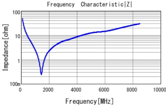
■ GRM1555C1H330GA01 |Z| DCOV, 25degC
