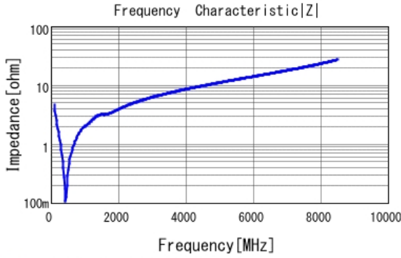
■ GRM1555C1H331JA01 |Z| DCOV, 25degC
