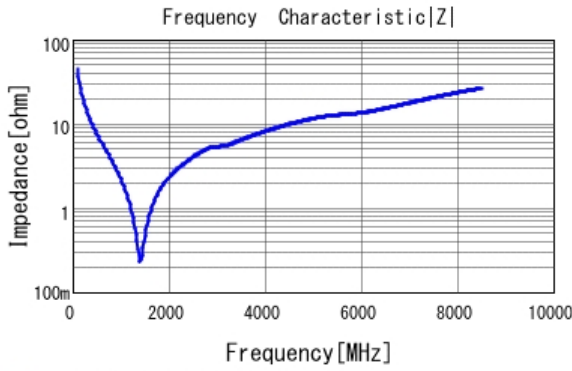
■ GRM1555C1H360JA01 |Z| DCOV, 25degC
