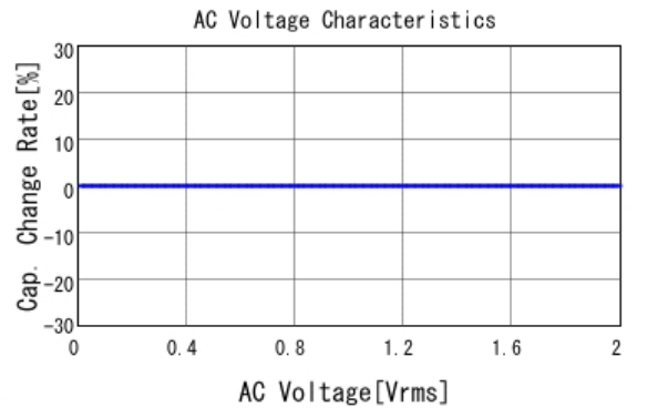
■ GRM1555C1H361JA01 C-AC Voltage capchange, DCOV, 25.0d
