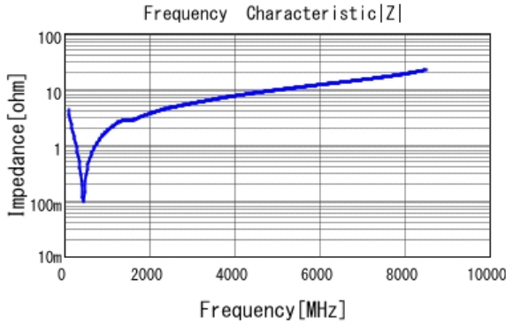
■ GRM1555C1H361JA01 |Z| DCOV, 25degC
