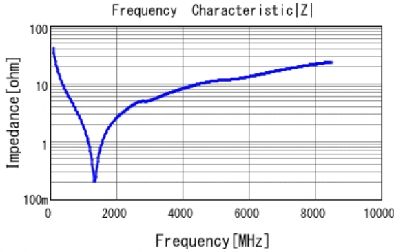
■ GRM1555C1H390JA01 |Z| DCOV, 25degC
