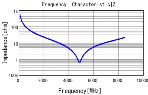
■ GRM1555C1H3R0CA01 |Z| DCOV, 25degC
