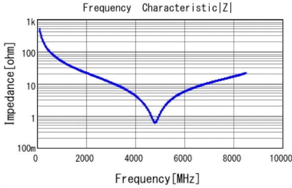
■ GRM1555C1H3R1WA01 |Z| DCOV, 25degC
