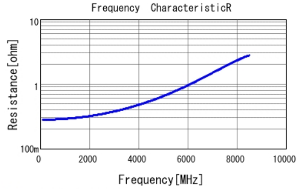
■ GRM1555C1H3R1WA01 R DCOV, 25degC
