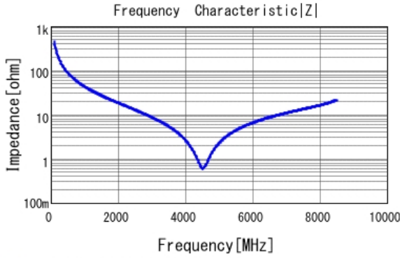
■ GRM1555C1H3R5BA01 |Z| DCOV, 25degC
