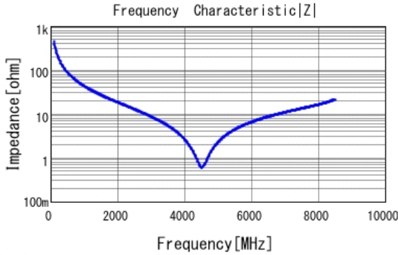
■ GRM1555C1H3R5WA01 |Z| DCOV, 25degC
