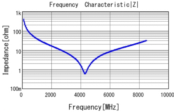
■ GRM1555C1H3R9BA01 |Z| DC0V, 25degC
