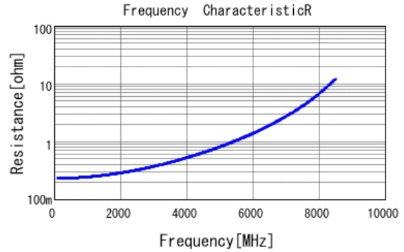
■ GRM1555C1H3R9BA01 R DC0V, 25degC
