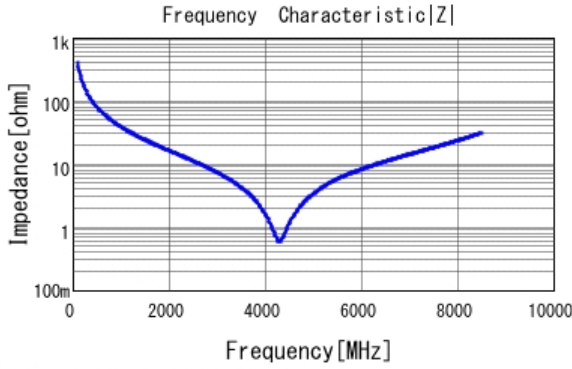
■ GRM1555C1H3R9WA01 |Z| DCOV, 25degC
