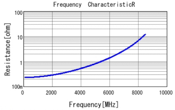
■ GRM1555C1H3R9WA01 R DCOV, 25degC
