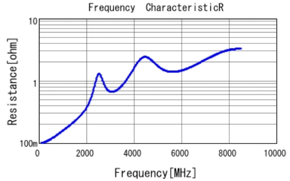
■ GRM1555C1H470GA01 R DCOV, 25degC
