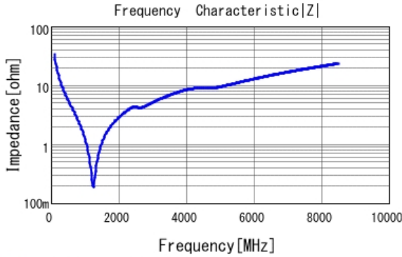
■ GRM1555C1H470GA01 |Z| DCOV, 25degC
