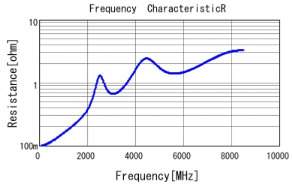
■ GRM1555C1H470JA01 R DCOV, 25degC
