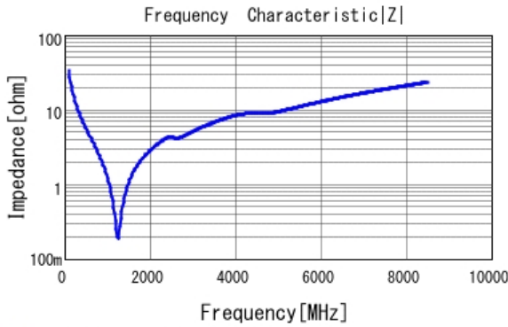
■ GRM1555C1H470JA01 |Z| DCOV, 25degC
