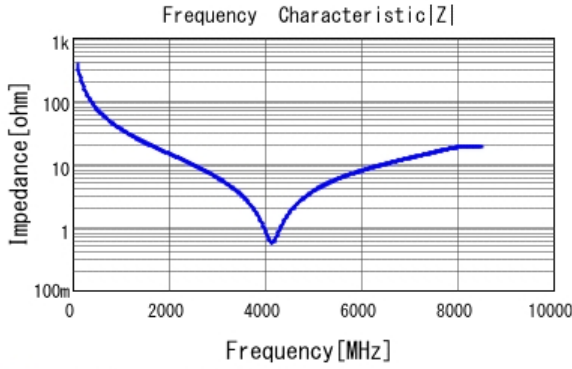
■ GRM1555C1H4R2CA01 |Z| DCOV, 25degC
