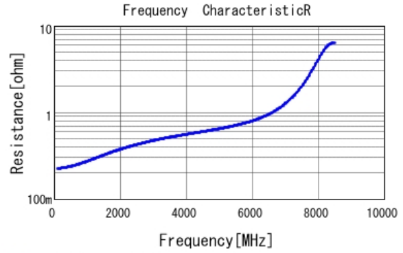
■ GRM1555C1H4R2CA01 R DCOV, 25degC
