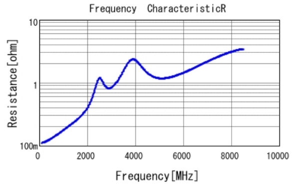
■ GRM1555C1H560JA01 R DCOV, 25degC
