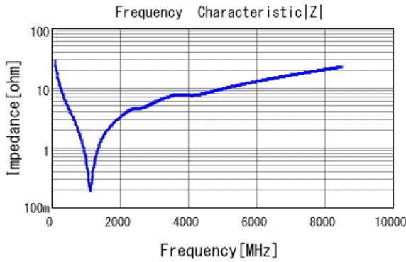
■ GRM1555C1H560JA01 |Z| DCOV, 25degC
