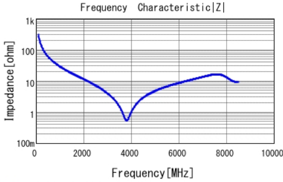
■ GRM1555C1H5R1BA01 |Z| DCOV, 25degC
