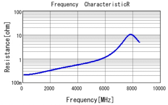
■ GRM1555C1H5R1BA01 R DCOV, 25degC
