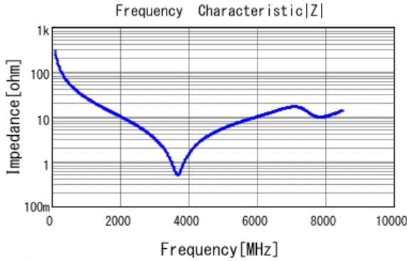
■ GRM1555C1H5R6BA01 |Z| DCOV, 25degC
