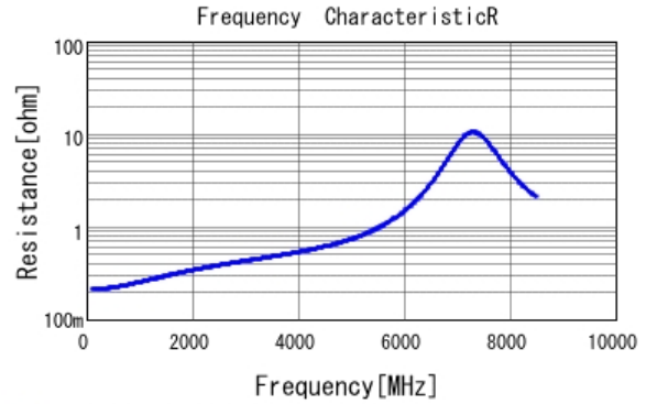
■ GRM1555C1H5R6BA01 R DCOV, 25degC
