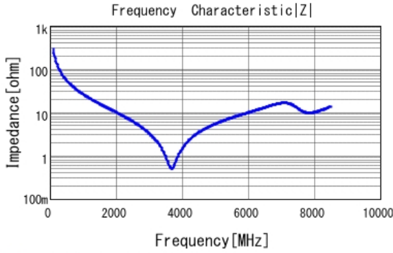
■ GRM1555C1H5R6CA01 |Z| DCOV, 25degC
