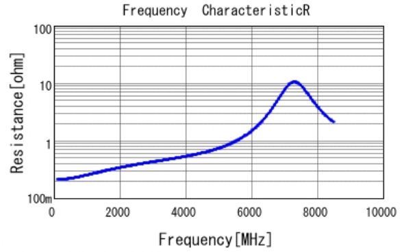
■ GRM1555C1H5R6CA01 R DCOV, 25degC
