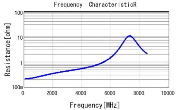
■ GRM1555C1H5R6DA01 R DCOV, 25degC
