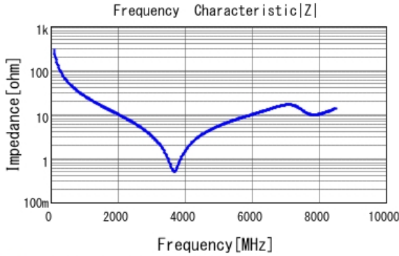
■ GRM1555C1H5R6DA01 |Z| DCOV, 25degC
