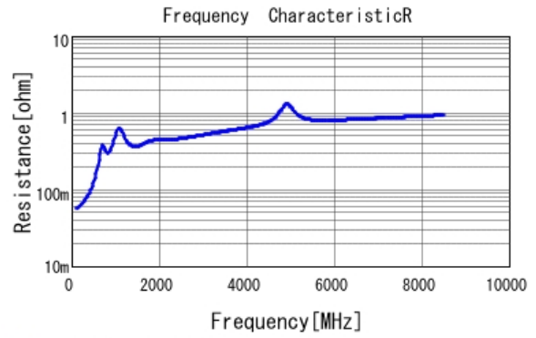
■ GRM1555C1H681JA01 R DCOV, 25degC
