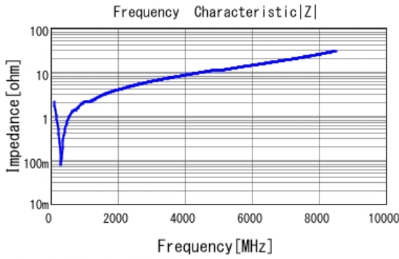
■ GRM1555C1H681JA01 |Z| DCOV, 25degC
