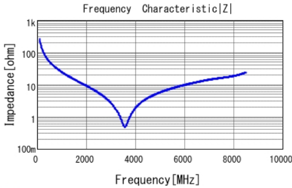
■ GRM1555C1H6R0CA01 |Z| DCOV, 25degC
