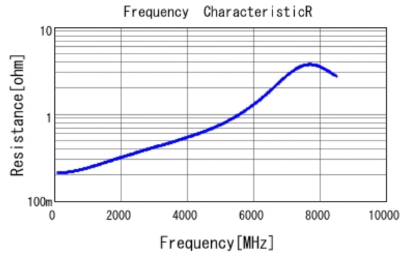
■ GRM1555C1H6R0DA01 R DCOV, 25degC
