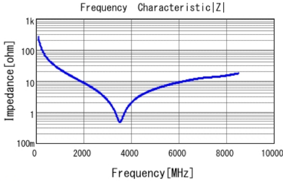
■ GRM1555C1H6R2CA01 |Z| DCOV, 25degC
