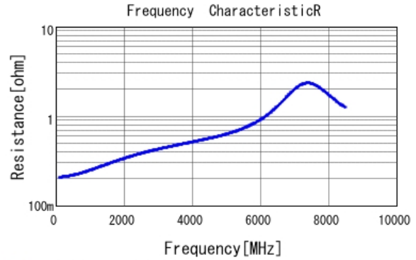
■ GRM1555C1H6R2CA01 R DCOV, 25degC
