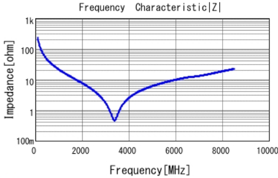
■ GRM1555C1H6R8CA01 |Z| DCOV, 25degC
