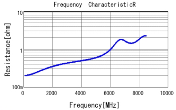
■ GRM1555C1H6R8CA01 R DCOV, 25degC
