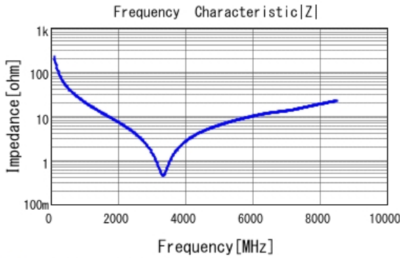
■ GRM1555C1H7R0CA01 |Z| DCOV, 25degC
