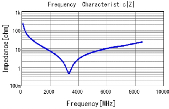
■ GRM1555C1H7R0DA01 |Z| DCOV, 25degC
