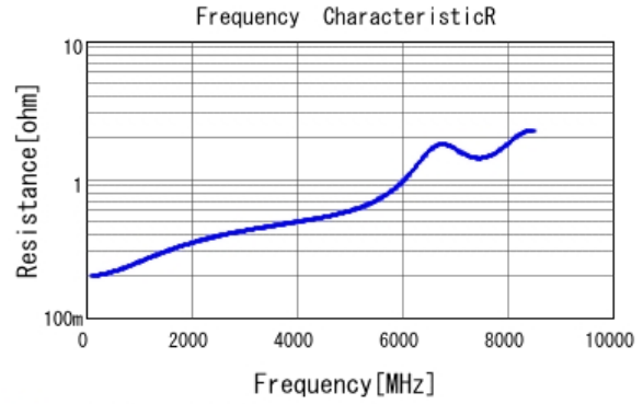
■ GRM1555C1H7R0DA01 R DCOV, 25degC
