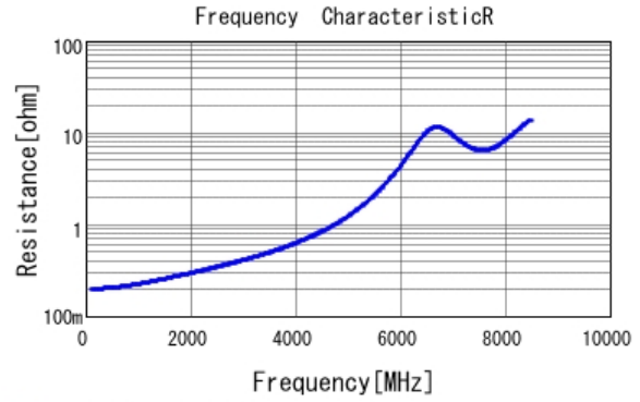
■ GRM1555C1H7R5CA01 R DC0V, 25degC
