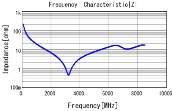
■ GRM1555C1H7R5CA01 |Z| DC0V, 25degC
