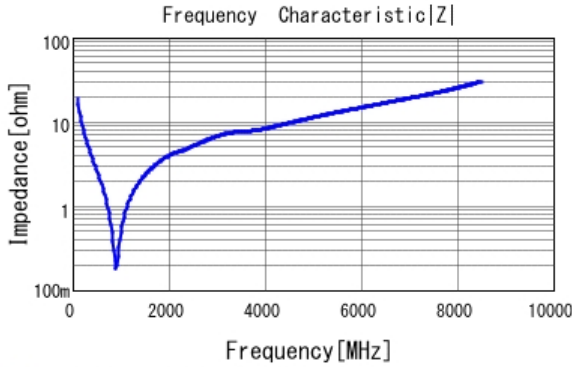
■ GRM1555C1H820JA01 |Z| DCOV, 25degC
