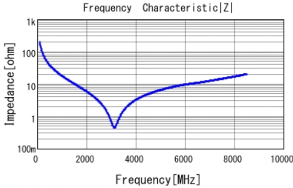
■ GRM1555C1H8R0CA01 |Z| DCOV, 25degC
