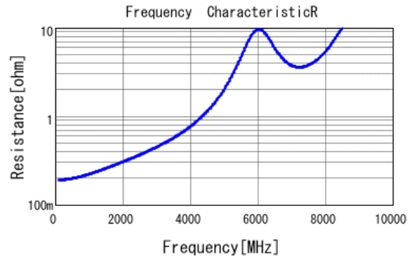
■ GRM1555C1H9R0BA01 R DCOV, 25degC
