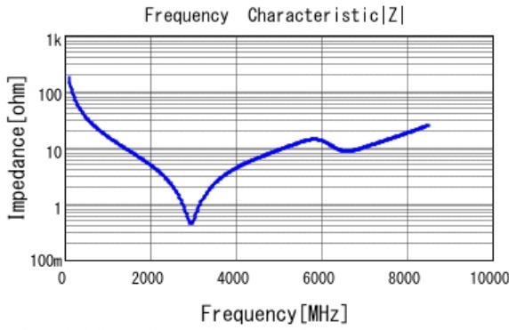
■ GRM1555C1H9R0BA01 |Z| DCOV, 25degC
