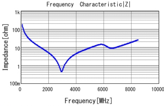
■ GRM1555C1H9R0WA01 |Z| DCOV, 25degC
