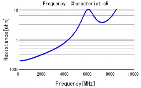
■ GRM1555C1H9R0WA01 R DCOV, 25degC
