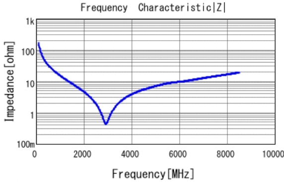
■ GRM1555C1H9R2CA01 |Z| DCOV, 25degC
