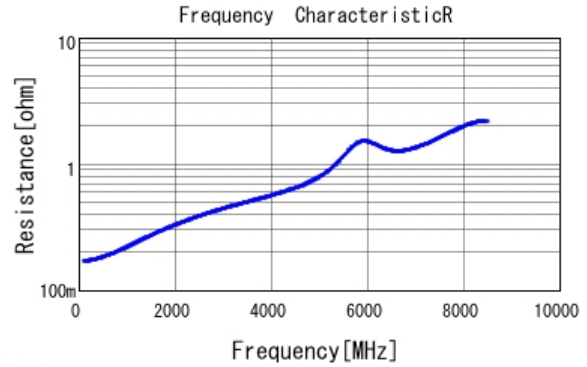
■ GRM1555C1H9R2CA01 R DCOV, 25degC
