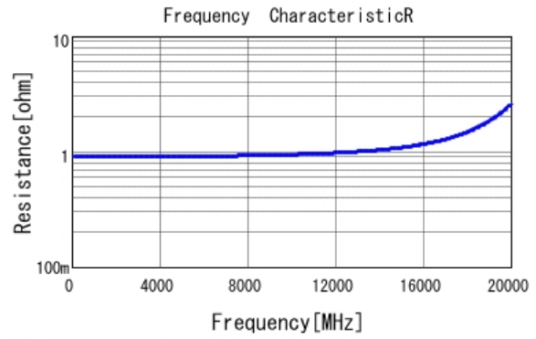
■ GRM1555C1HR30BA01 R DCOV, 25degC
