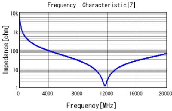
■ GRM1555C1HR40WA01 |Z| DCOV, 25degC
