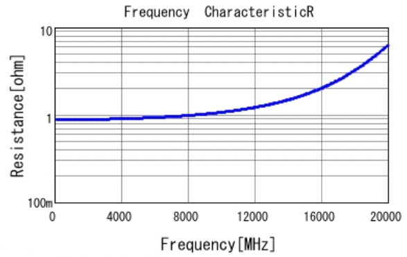
■ GRM1555C1HR40WA01 R DCOV, 25degC
