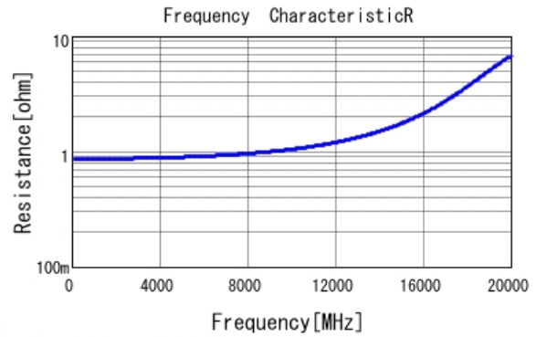
■ GRM1555C1HR50BA01 R DCOV, 25degC
