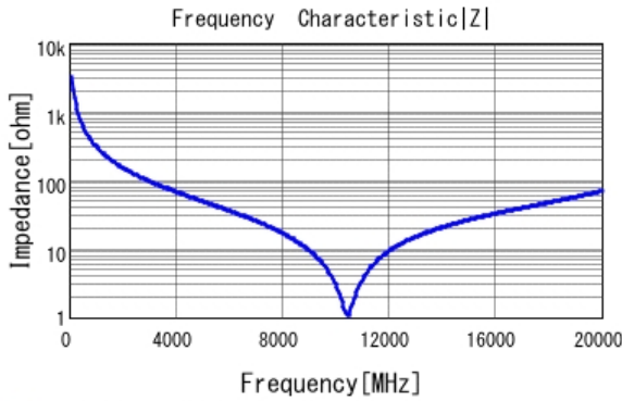
■ GRM1555C1HR50BA01 |Z| DCOV, 25degC
