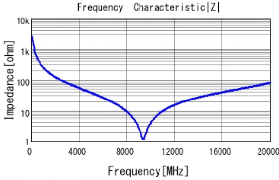
■ GRM1555C1HR60BA01 |Z| DCOV, 25degC
