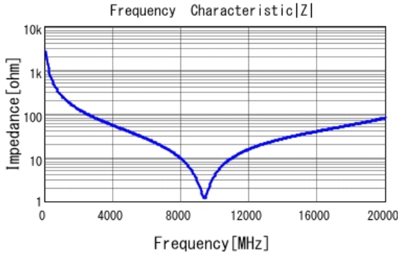
■ GRM1555C1HR60WA01 |Z| DCOV, 25degC
