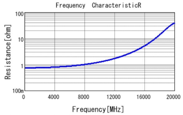
■ GRM1555C1HR90WA01 R DCOV, 25degC
