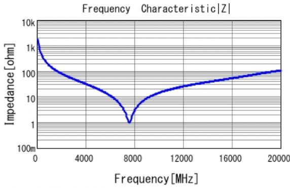
■ GRM1555C1HR90WA01 |Z| DCOV, 25degC
