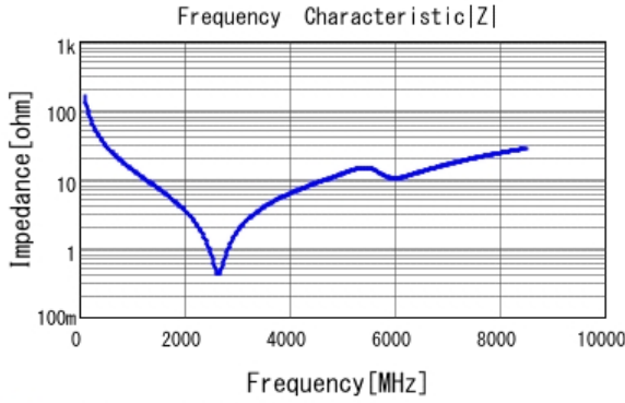
■ GRM1555C2A100JA01 |Z| DCOV, 25degC
