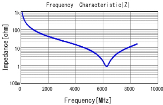
■ GRM1555C2A1R8WA01 |Z| DCOV, 25degC
