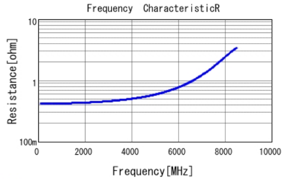
■ GRM1555C2A1R8WA01 R DCOV, 25degC
