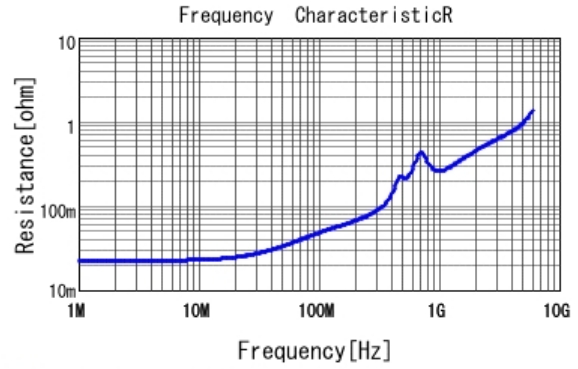
■ GRM1557U1A152JA01 R DCOV, 25degC
