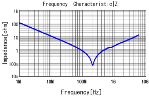
■ GRM1557U1A152JA01 |Z| DCOV, 25degC
