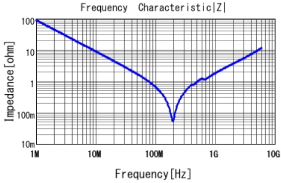
■ GRM1557U1A182JA01 |Z| DCOV, 25degC
