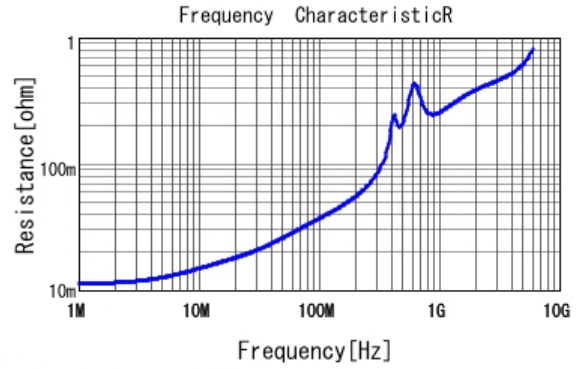
■ GRM1557U1A182JA01 R DCOV, 25degC
