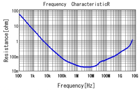
■ GRM155B10J224KE01 R DCOV, 20degC
