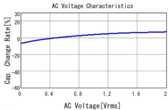
■ GRM155B10J224KE01 C-AC Voltage capchange, DCOV, 20.0d
