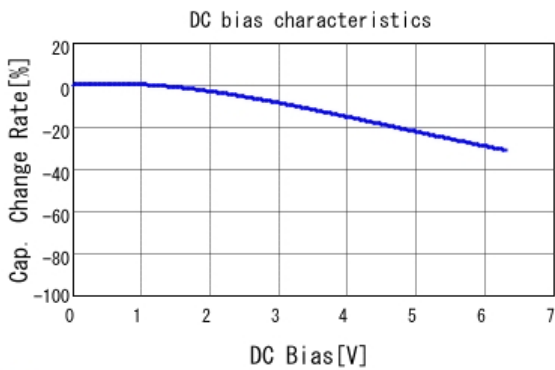
■ GRM155B10J224KE01 C-DC bias capchange, 20.0degC, AC0.
