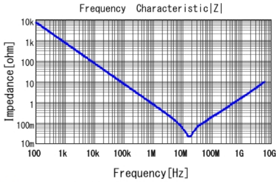
■ GRM155B10J224KE01 |Z| DCOV, 20degC
