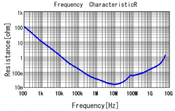
■ GRM155B11A104KA01 R DCOV, 20degC
