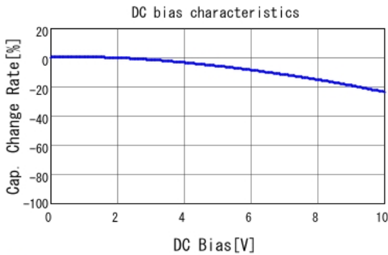
■ GRM155B11A104KA01 C-DC bias capchange, 20.0degC, AC1.
