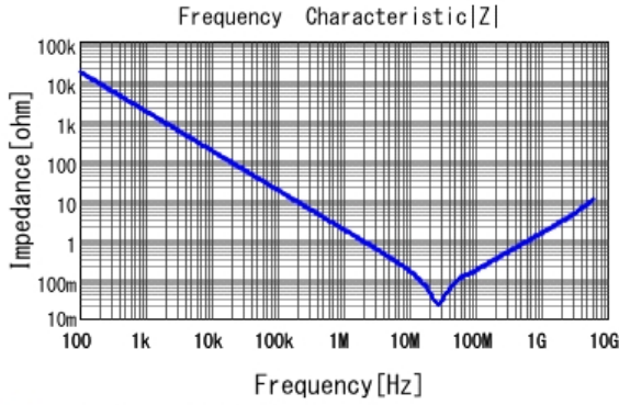
■ GRM155B11A104KA01 |Z| DCOV, 20degC
