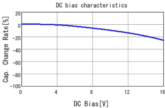
■ GRM155B11C473KA01 C-DC bias capchange, 20.0degC, AC1.
