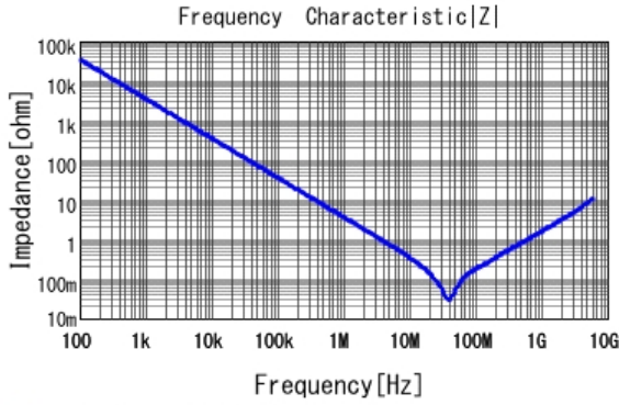
■ GRM155B11C473KA01 |Z| DCOV, 20degC
