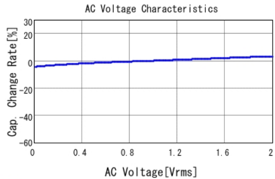
■ GRM155B11C473KA01 C-AC Voltage capchange, DCOV, 20.0d
