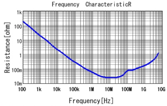
■ GRM155B11C473KA01 R DCOV, 20degC
