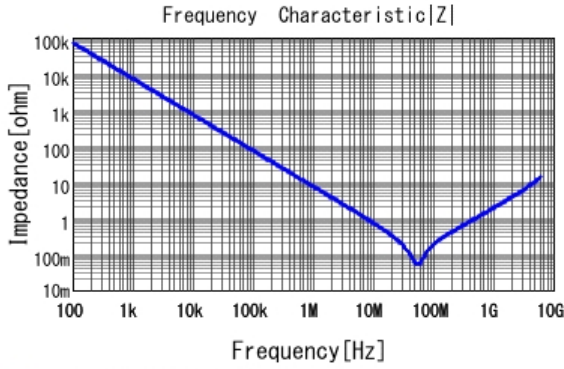
■ GRM155B11E223KA61 |Z| DCOV, 20degC
