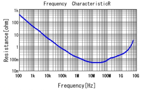
■ GRM155B11E223KA61 R DCOV, 20degC
