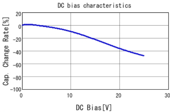
■ GRM155B11E223KA61 C-DC bias capchange, 20.0degC, AC1.
