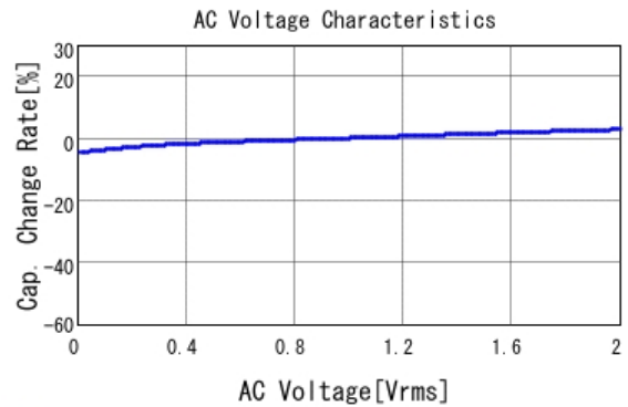
■ GRM155B11E223KA61 C-AC Voltage capchange, DCOV, 20.0d
