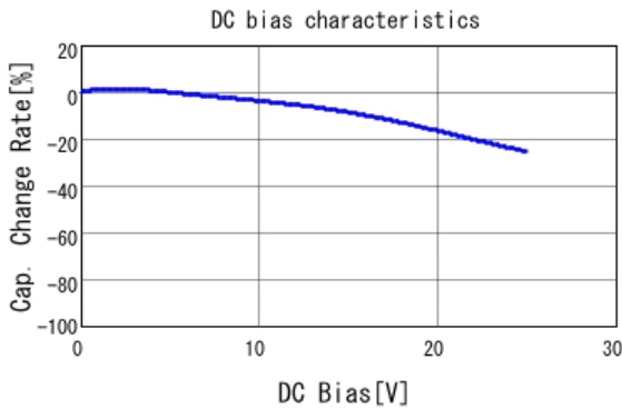
■ GRM155B11E682KA01 C-DC bias capchange, 20.0degC, AC1.
