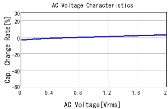
■ GRM155B11E682KA01 C-AC Voltage capchange, DCOV, 20.0d
