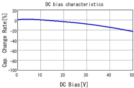
■ GRM155B11H331KA01 C-DC bias capchange, 20.0degC, AC1.
