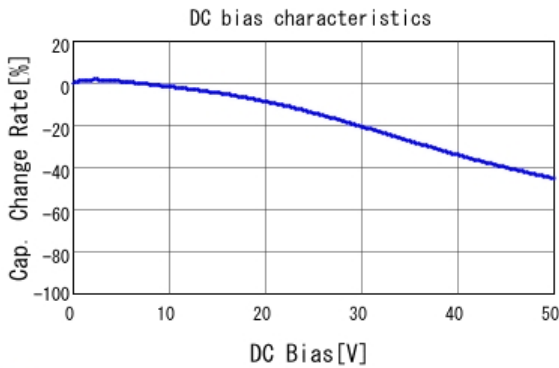
■ GRM155B11H332KA01 C-DC bias capchange, 20.0degC, AC1.
