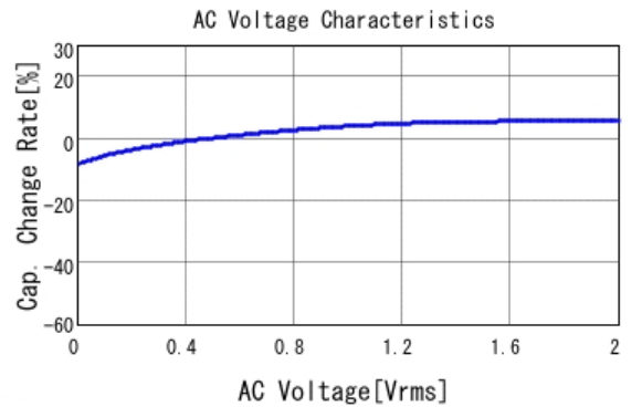
■ GRM155B30J474KE18 C-AC Voltage capchange, DCOV, 20.0d
