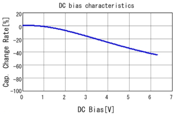
■ GRM155B30J474KE18 C-DC bias capchange, 20.0degC, AC0.
